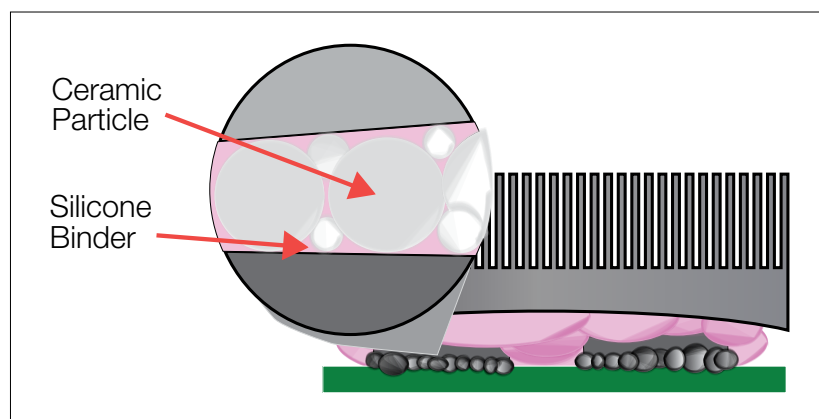
Figure 2: Electrical Isolation
